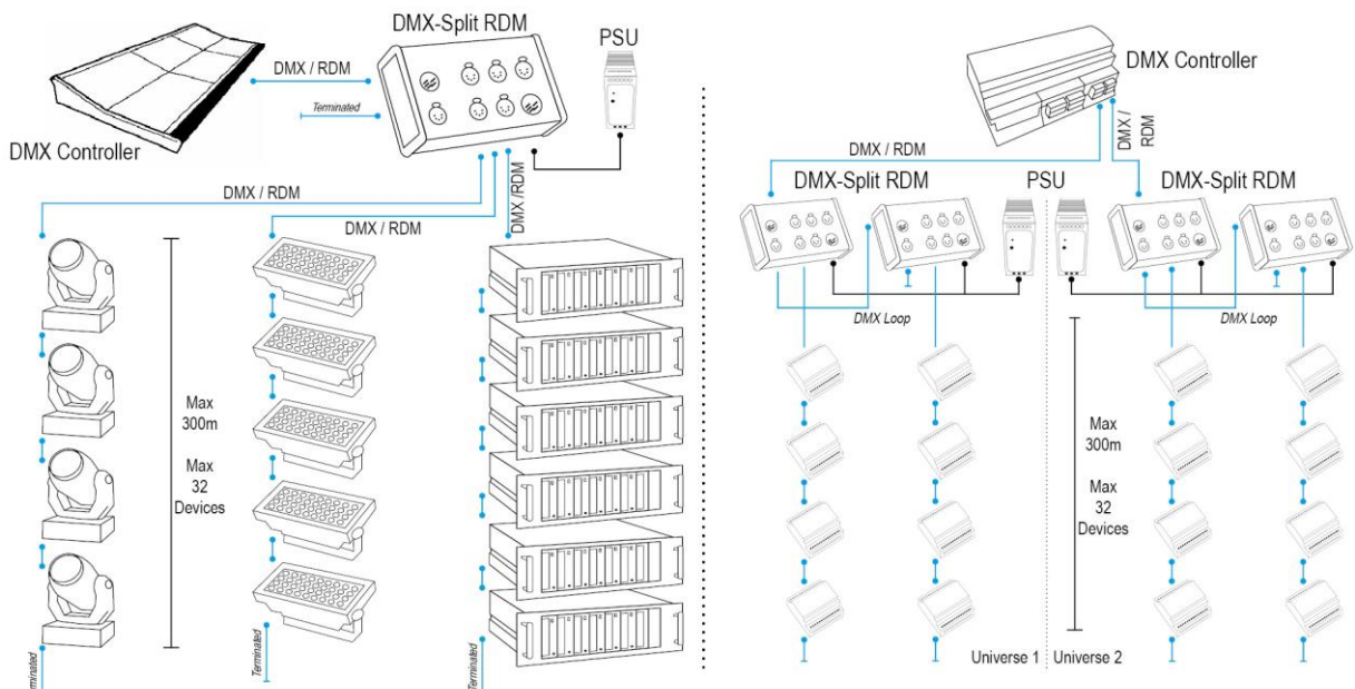
Single Universe, Single DMX Splitter
